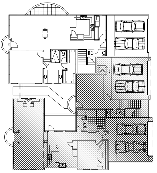
Unit Plan, First Floor
